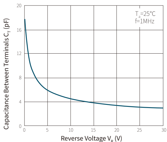
Fig.3 Capacitance Characteristics
