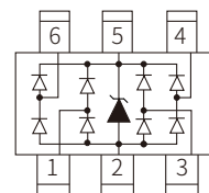
Schematic Symbol
