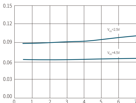
Figure 4: Drain-Source On-Resistance
