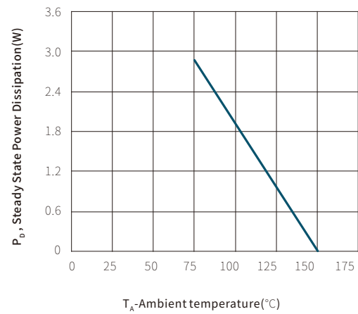
Steady State Power Dissipation Derating Curve
