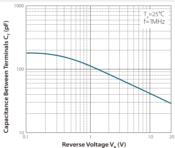
Fig.3 Capacitance Characteristics
