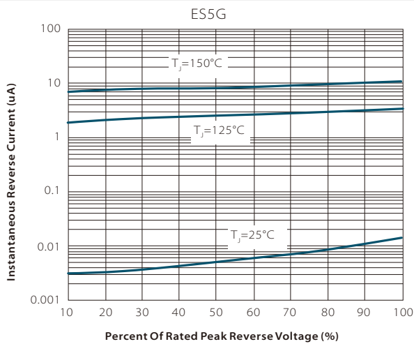
Fig. 5-Typical Reverse Characteristics
