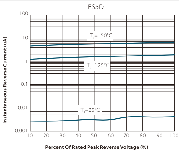
Fig. 3-Typical Reverse Characteristics
