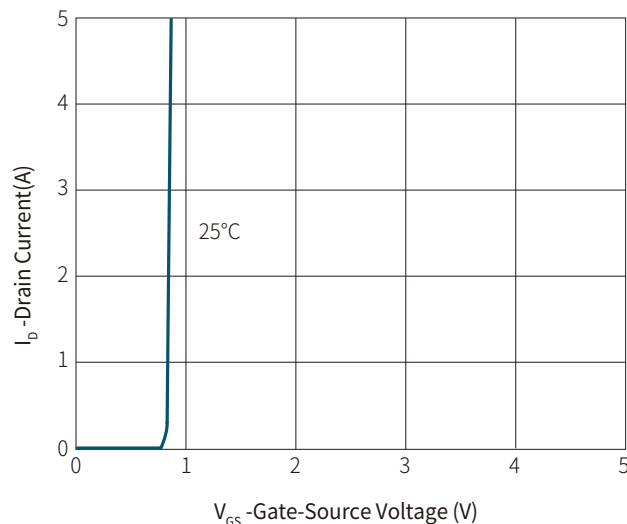
Figure2: Transfer Characteristic
