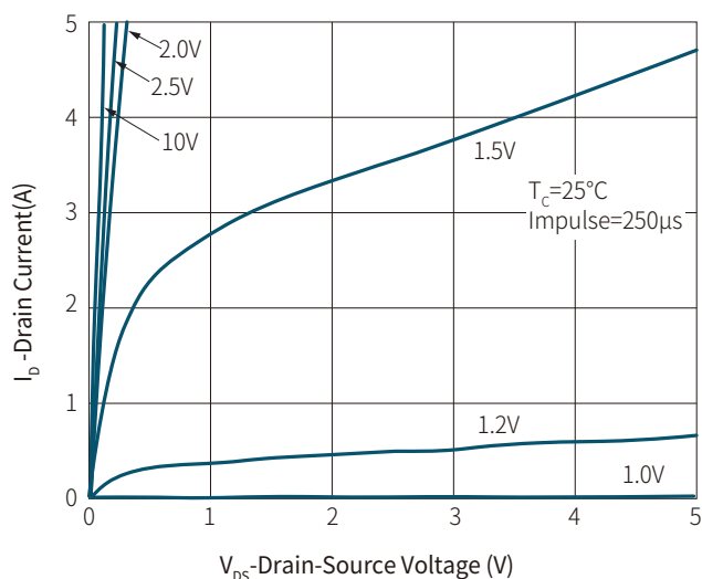
Figure1: Output Characteristic
