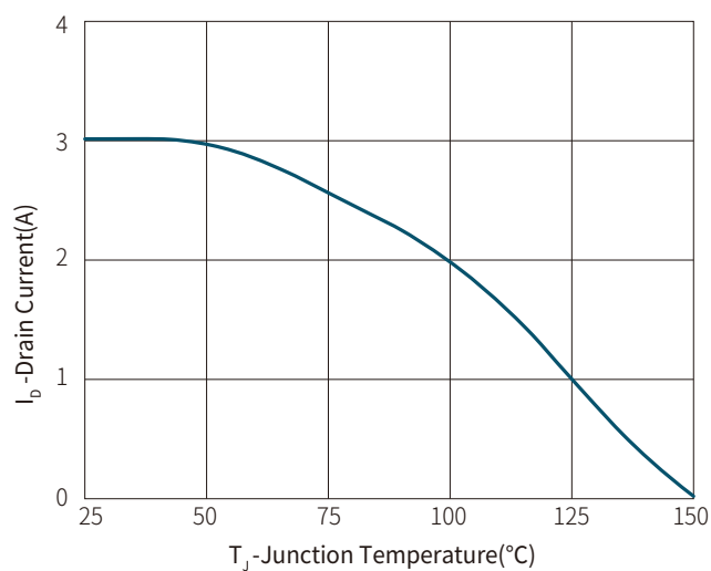
Figure 10: Maximum PContinuous Drain Current vs Case Temperature
