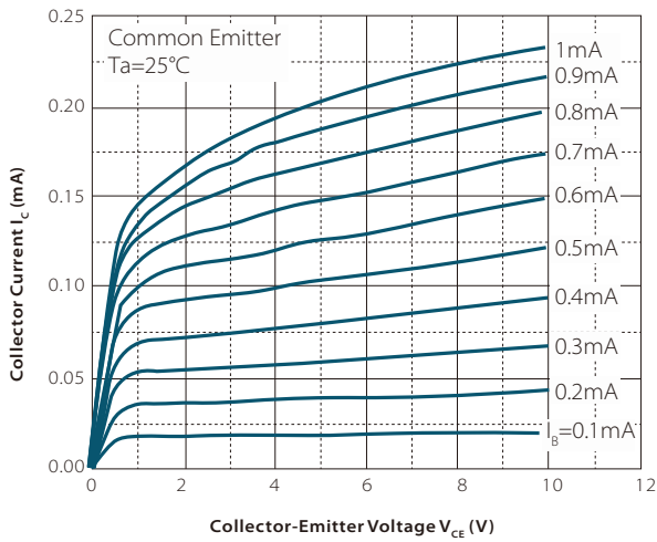
Static Characteristic
