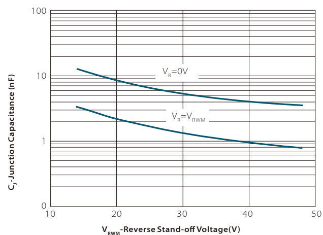
Fig.6 Typical Capacitance
