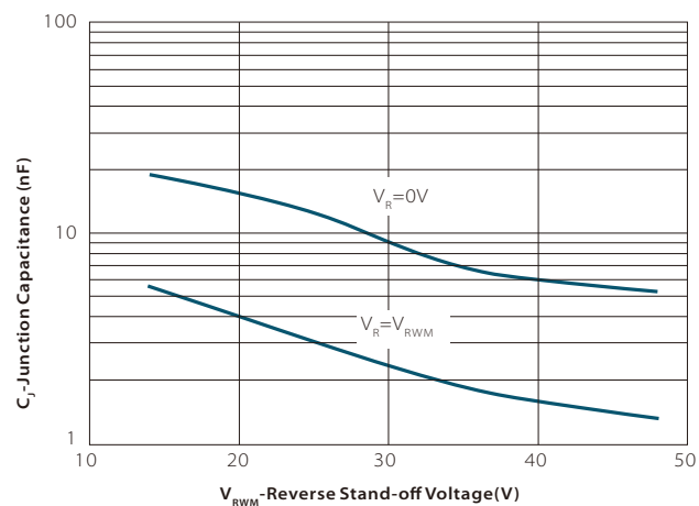
Fig.6 Typical Capacitance
