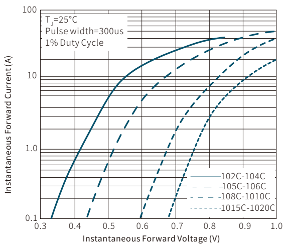
Fig. 3-Forward Voltage
